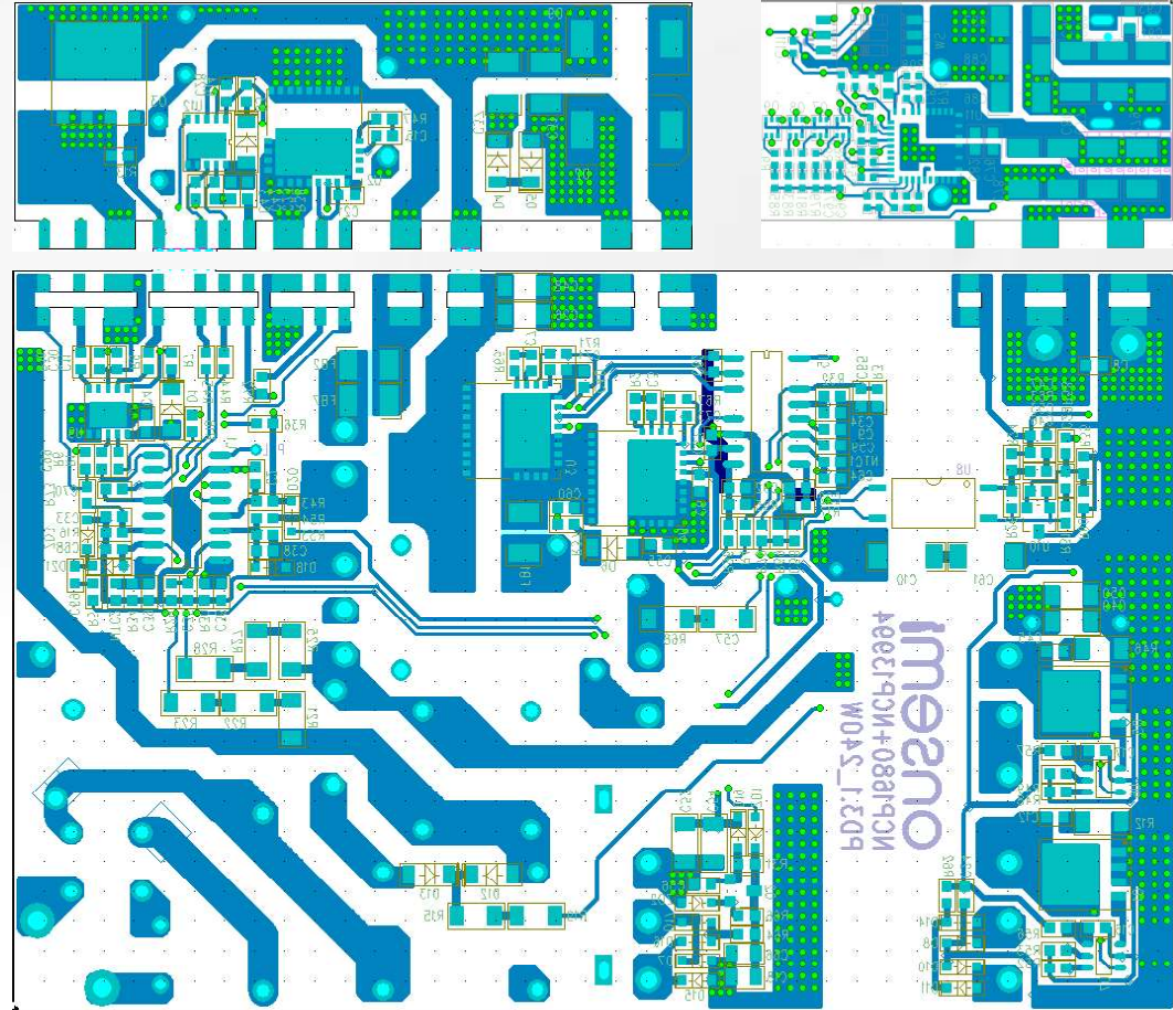
Bottom Layout
