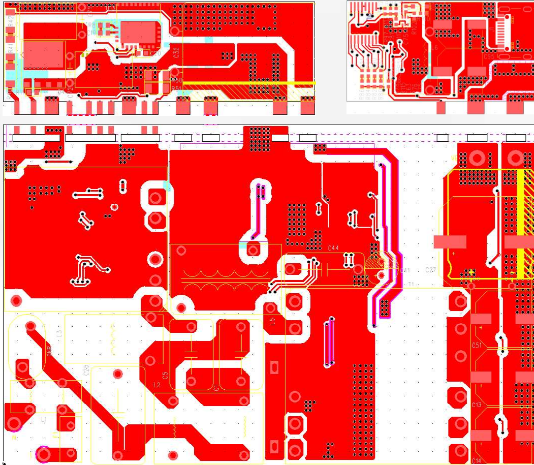
Top Layout
