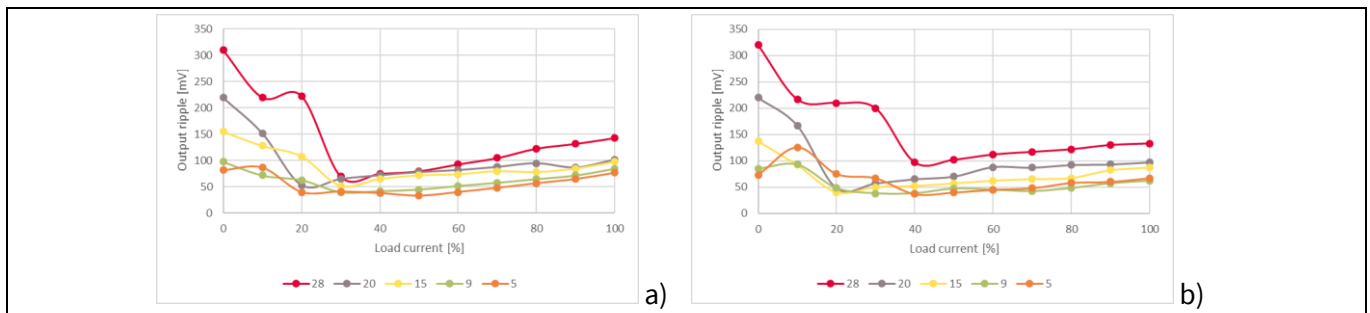
Figure 23 Output ripple measured at Type-C connector: a) 115 V AC and b) 230 V AC
