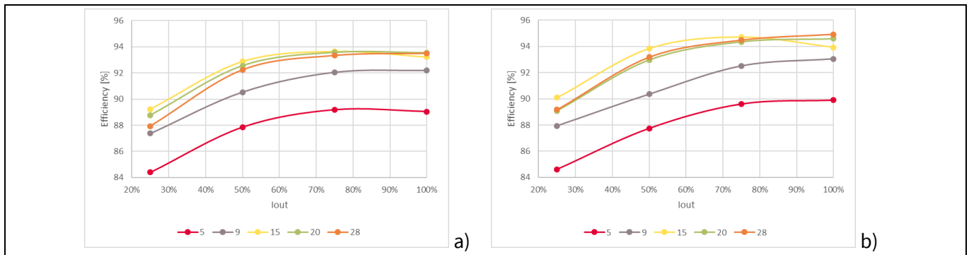
Figure 24 Efficiency measured at the Type-C connector: a) 115 V AC and b) 230 V AC
