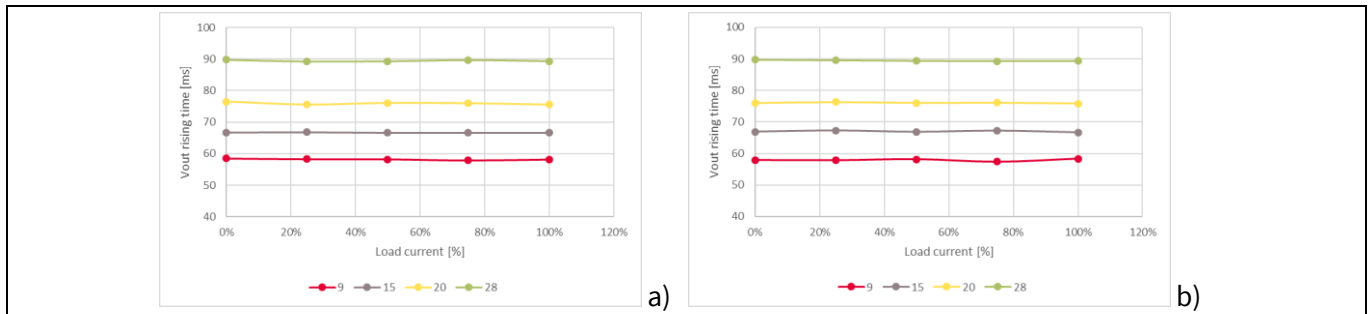
Figure 21 Output voltage rising time from 5 V to other voltage levels: a) 115 V AC and b) 230 V AC
