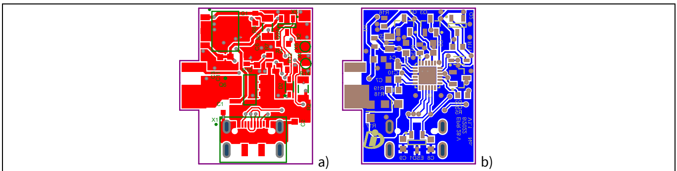
Figure 12 EPR board PCB: a) top side and b) bottom side
