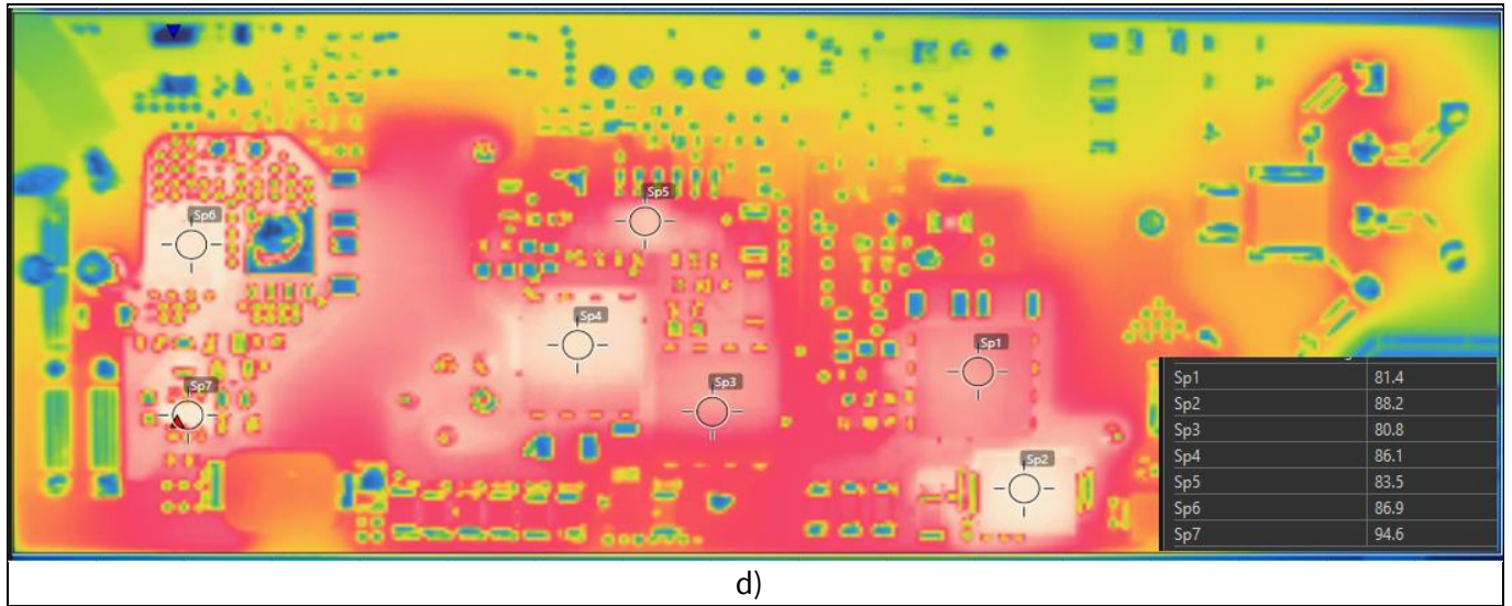
Figure 29 Thermal measurement: a) top side at 115 V AC, b) bottom side at 115 V AC, c) top side at 230 V AC and d) bottom side at 230 V AC
