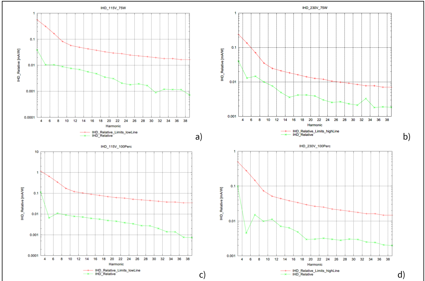
Figure 16 Harmonics current (green line) and its limit from IEC 61000-3-2 (red line): a) 115 V AC, 75 W, b) 230 V AC, 75 W, c) 115 V AC, 140 W and d) 230 V AC, 140 W
