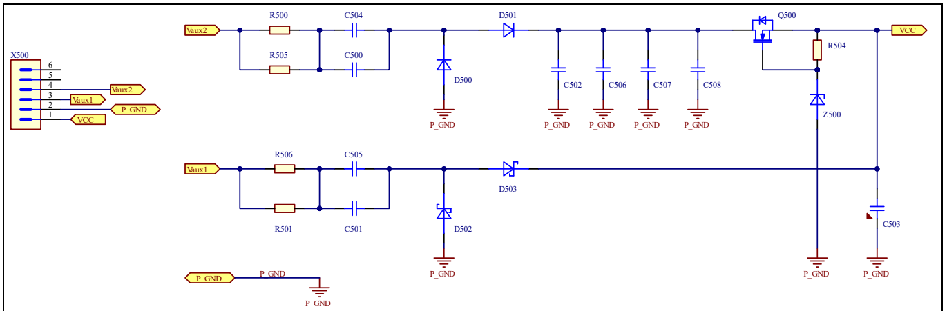
Figure 9 V CC board schematic
