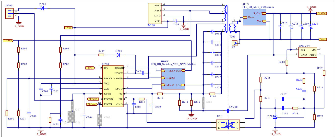
Figure 4 HFB stage schematic
