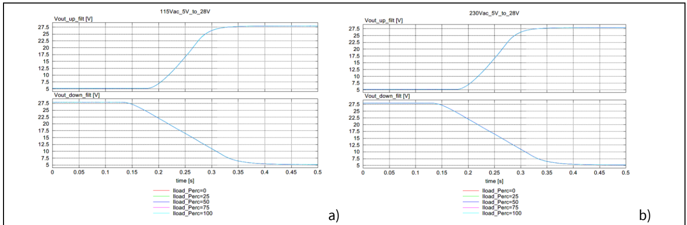
Figure 20 Output voltage transition between 5 V and 28 V: a) 115 V AC and b) 230 V AC
