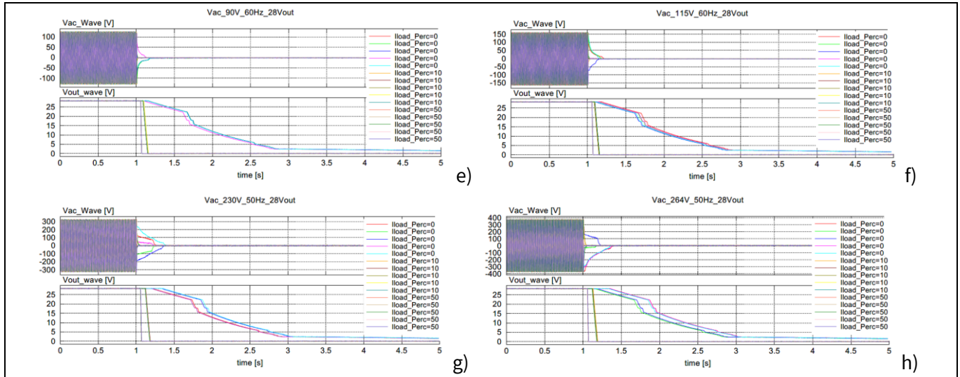
Figure 27 X-capacitor discharge
