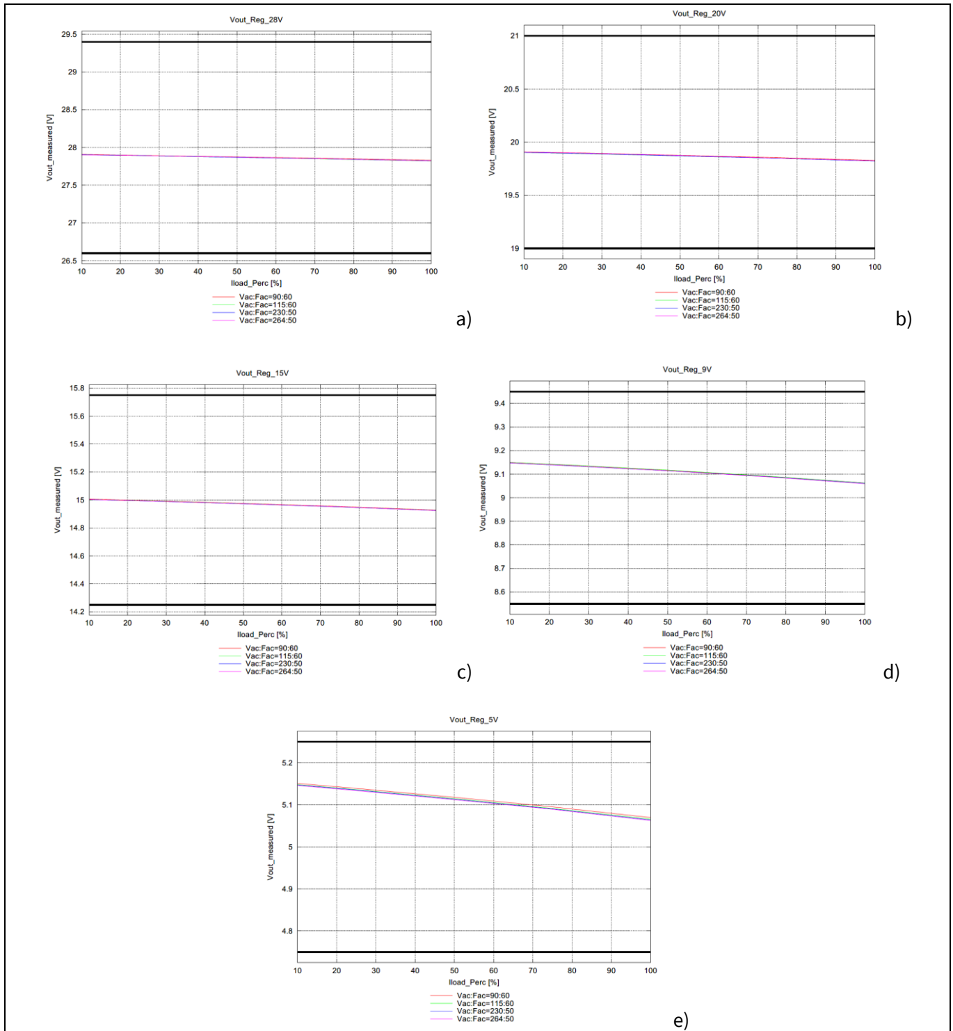
Figure 18 Output voltage in steady-state operation measured at the Type-C connector: a) 28 V, b) 20 V, c) 15 V, d) 9 V and e) 5 V
