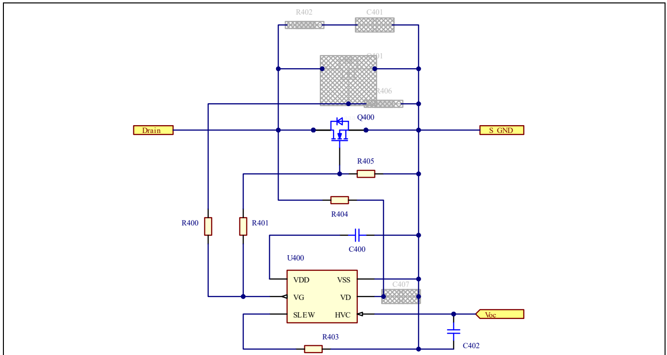
Figure 6 Synchronous rectification schematic
