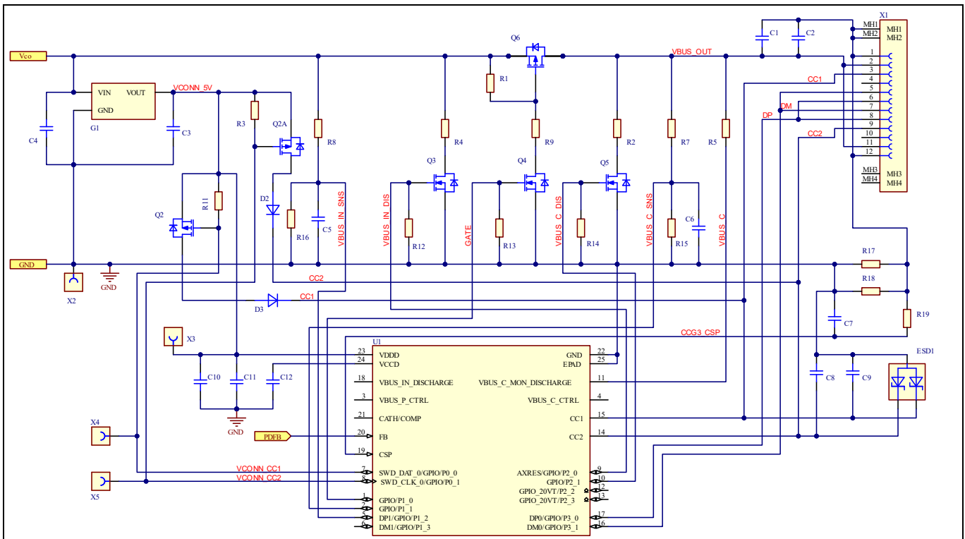
Figure 11 EPR board schematic
