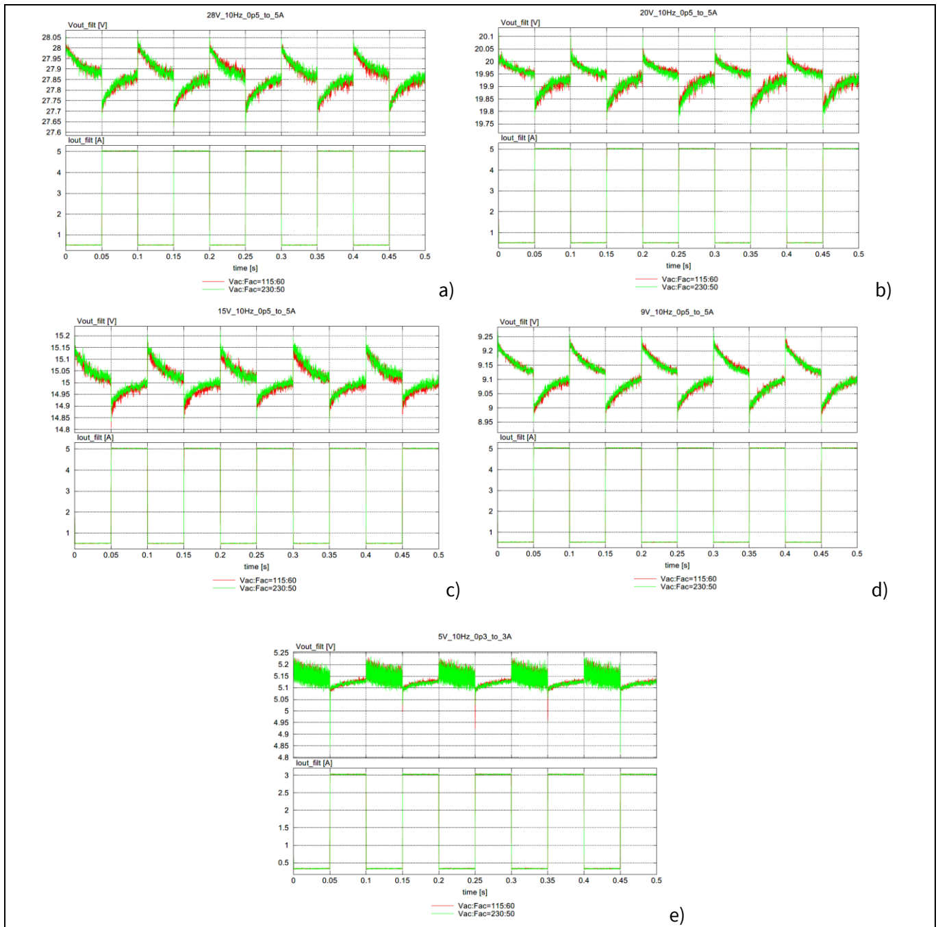
Figure 19 Output voltage at dynamic load current between 10 percent and 100 percent, measured at the HFB output capacitor: a) 28 V, b) 20 V, c) 15 V, d) 9 V and e) 5 V
