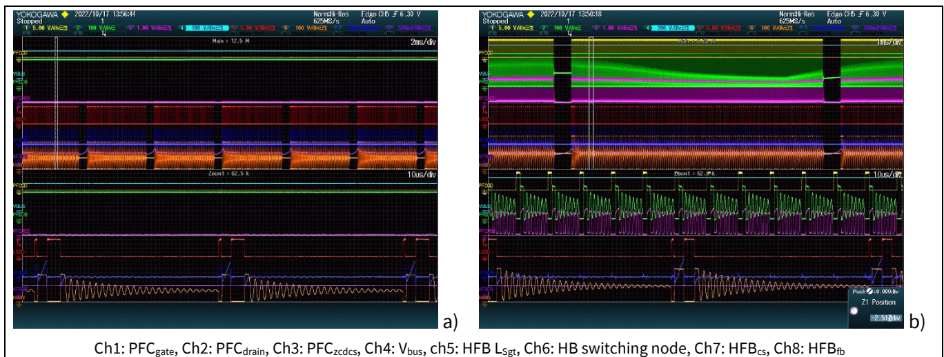
Figure 13 Waveform in burst mode operation: HFB in ZV-RVS with a) PFC disabled at 230 V input and 20 V, 0.15 A output, and b) PFC enabled at 115 V input and 28 V, 0.15 A output
