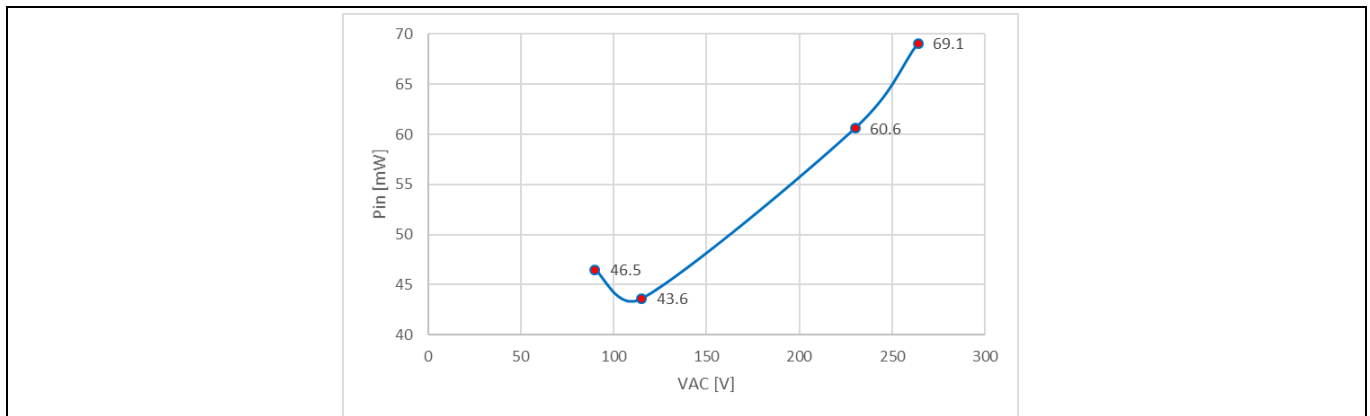
Figure 26 Standby input power measurement with EPR board disconnected
