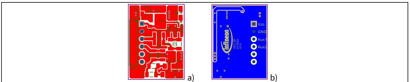
Figure 10 PCB of the V CC board: a) top side and b) bottom side
