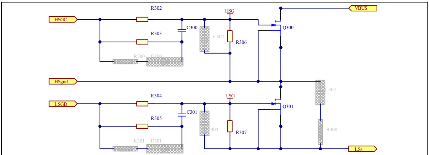
Figure 5 Half-bridge and gate RC network schematic
