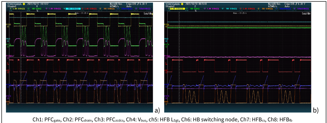
Figure 15 Continuous operation mode with HFB in ZV-RVS mode: a) PFC switching at third valley at 115 V input and 28 V 2 A output, and b) PFC disabled at 230 V, 15V 1 A output
