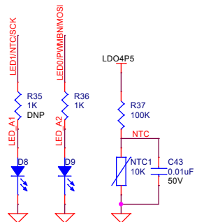
LED&NTC
