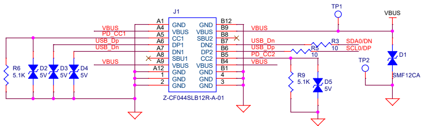
POWER INPUT
