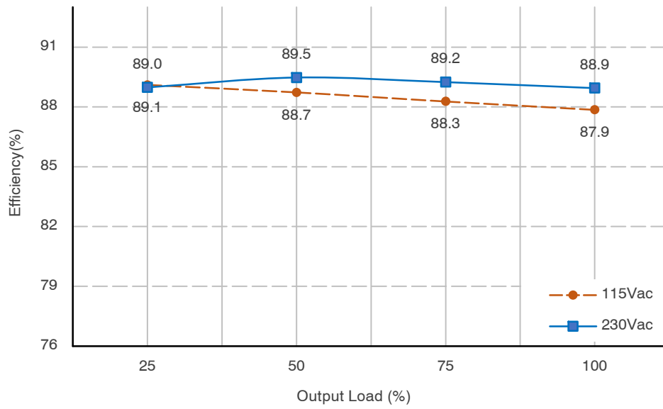
Figure 8. Efficiency at 4 Points Load
