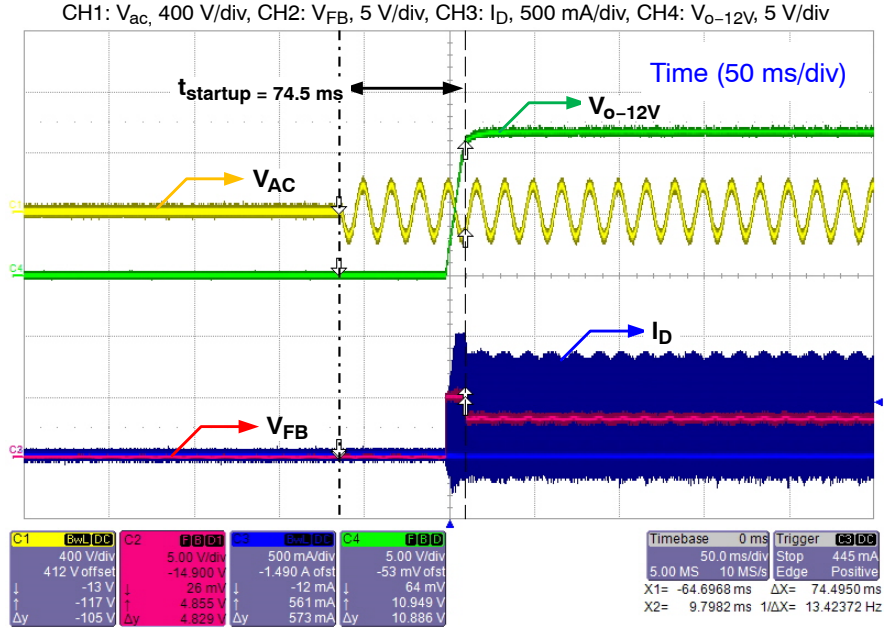
Figure 14. Star-up Operation @ 115 V_{ac} /60 Hz, Full Load
