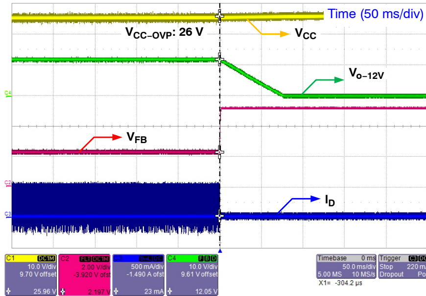
Figure 30. V_{CC} OVP @ 230 V_{ac} /60 Hz, Full Load
