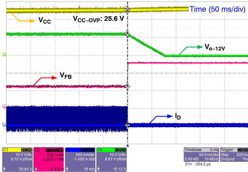
Figure 29. V_{CC} OVP @ 115 V_{ac} /60 Hz, Full Load
