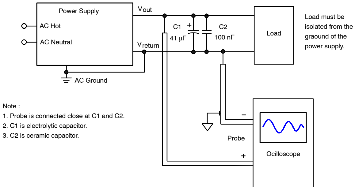
Figure 18. Test Method for Output Ripple and Noise
