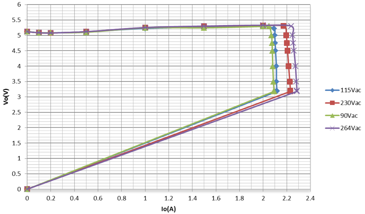
Figure 7. I-V Curves
