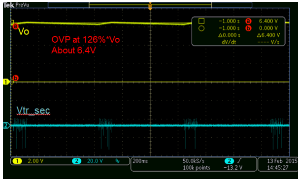
Figure 14. Test Condition: 264 Vac, No Dummy Load
