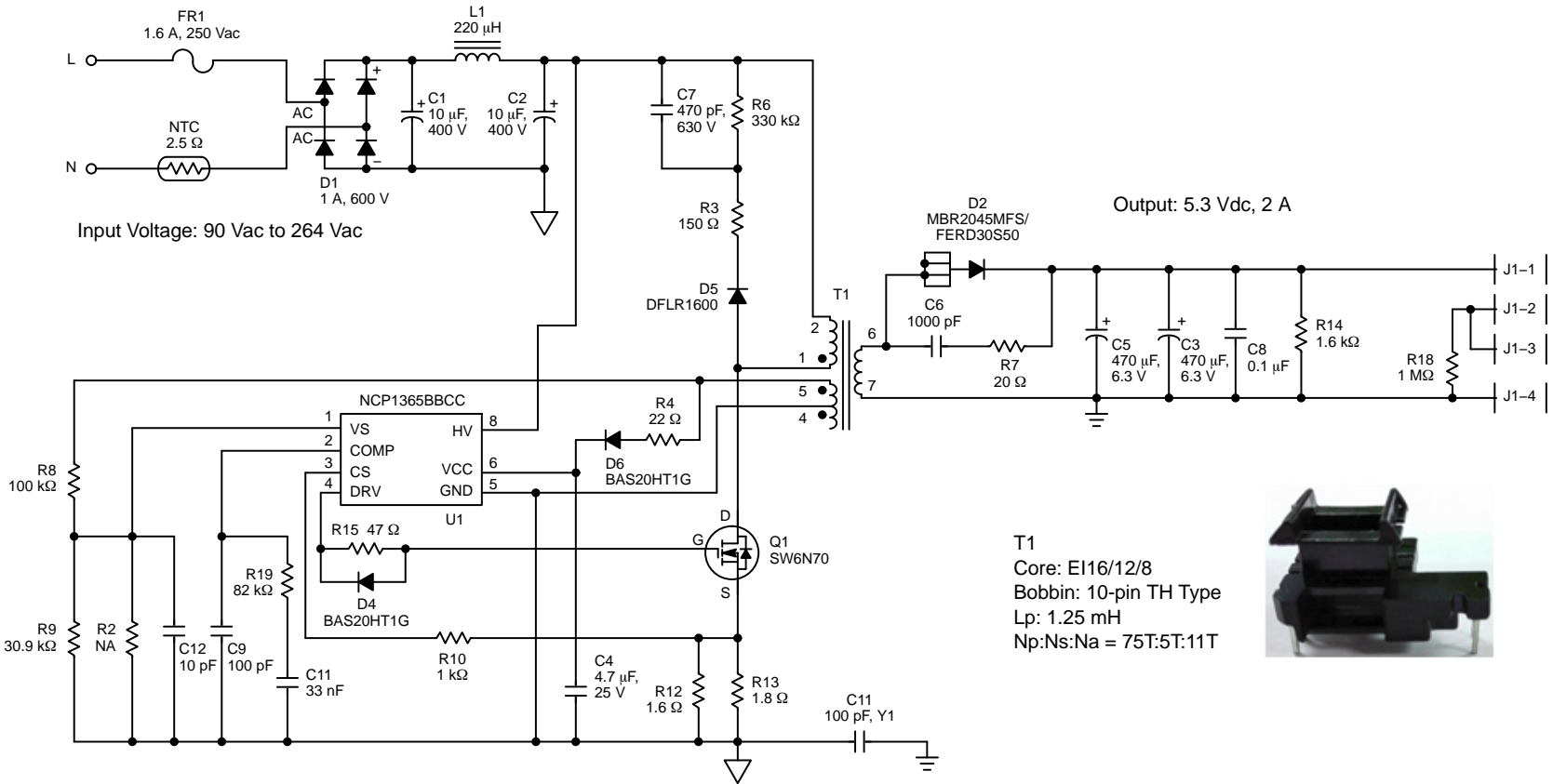
Figure 3. Circuit Schematic
