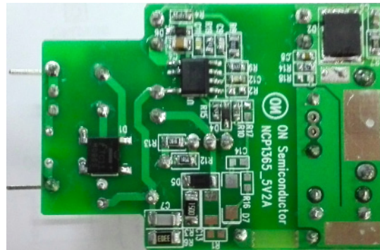
Figure 2. Demoboard Photo
