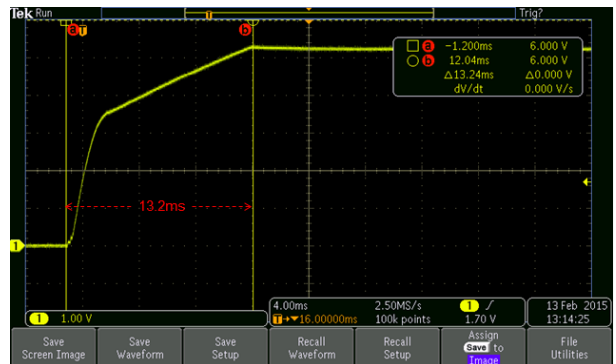
Figure 19. 230 Vac and 2 A CC Load
