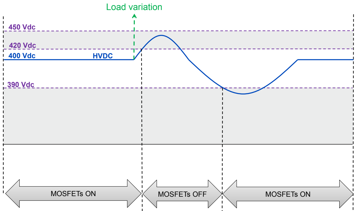
Figure 51. Overvoltage protection
