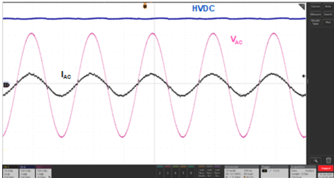
Figure 66. PFC steady state with V_{AC} = 230 V_{RMS}/50 Hz and P_{out} = 2 kW
