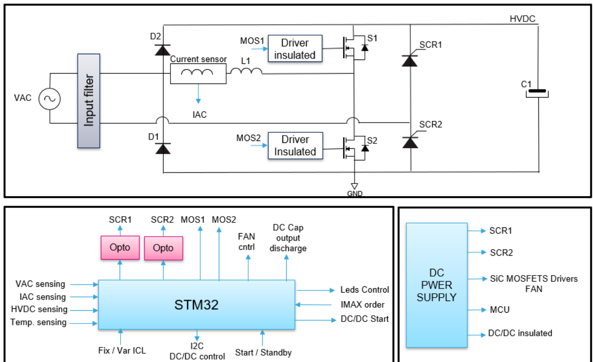
Figure 13. Bridgeless PFC totem pole synaptic
