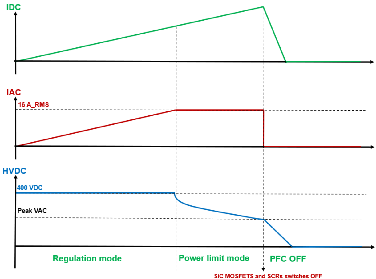
Figure 49. Over input current protection
