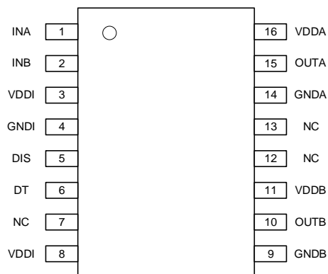
Figure 1.2 NSi6602 SOW16/SOP16 Package
